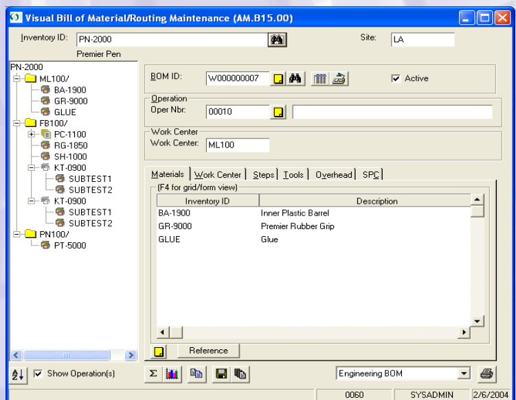
The Visual Bill of Material/Routing Maintenance Screen allows for easy creation and maintenance of key fields.
